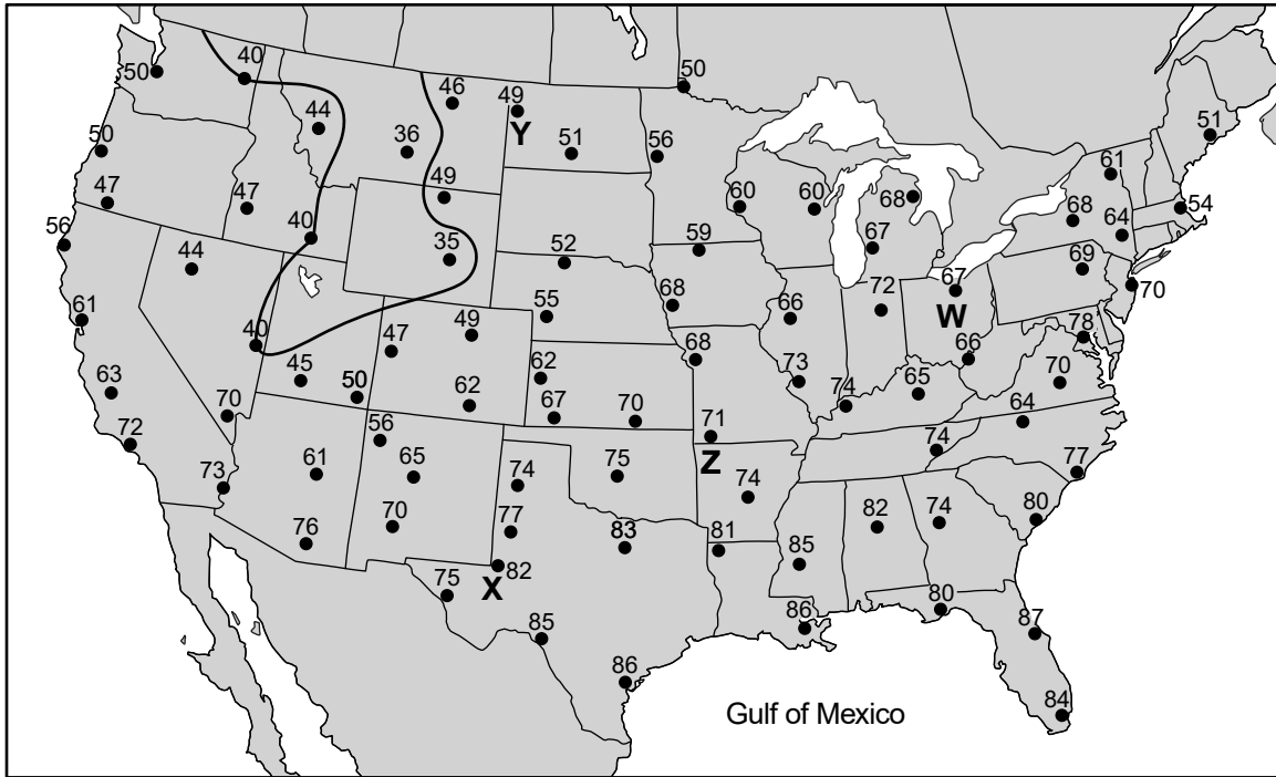
Surface Air Temperature (°F) October 25, 2010
