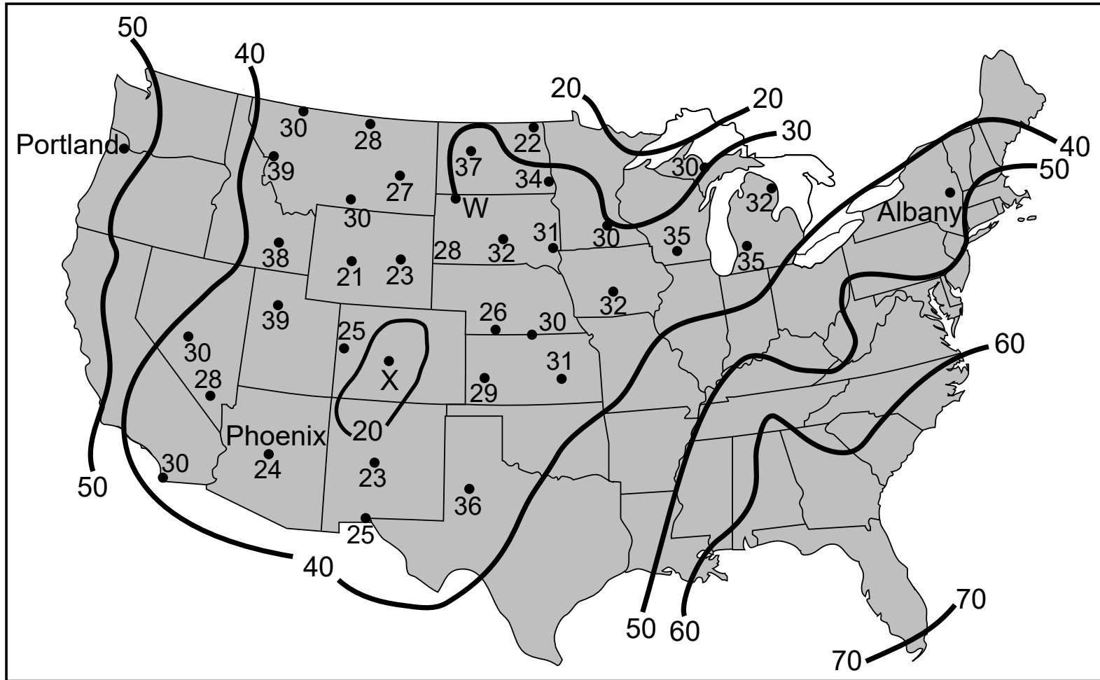
Dewpoint Isoline Map - 3:00 p.m. November 1, 2018
