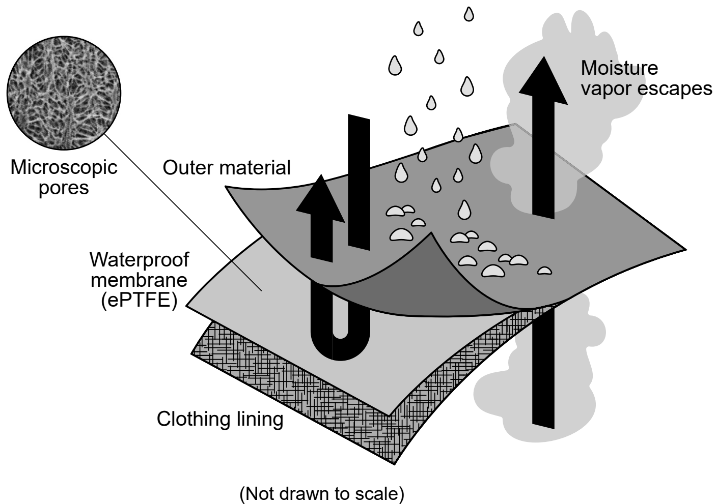
Figure 1: Waterproof Clothing Layers
