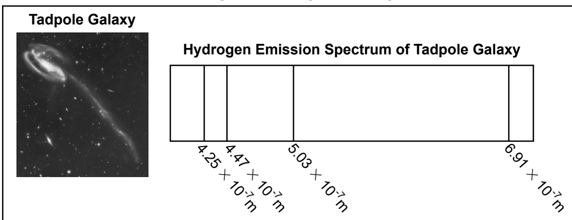
Diagram 2: Tadpole Galaxy
