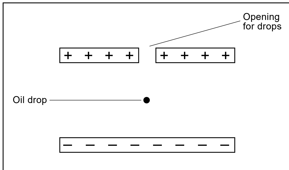
Diagram 1: Millikan's Oil Drop Experiment Simulation
