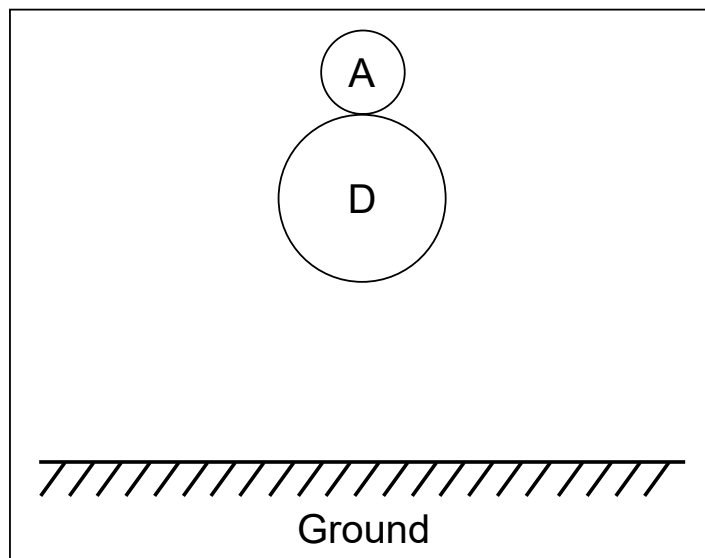
Diagram 3: Ball A on Top of Ball D
