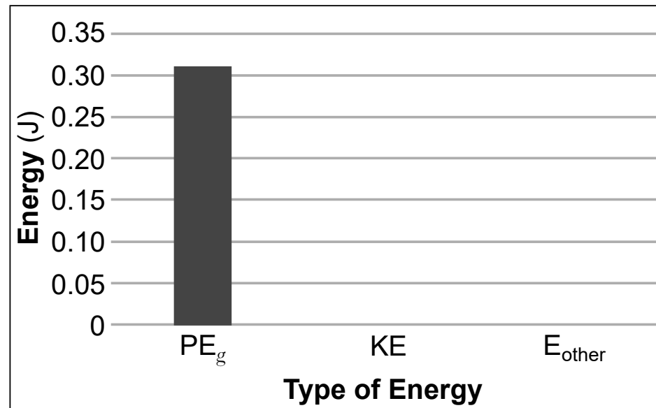
Graph 1: Types of Energy
