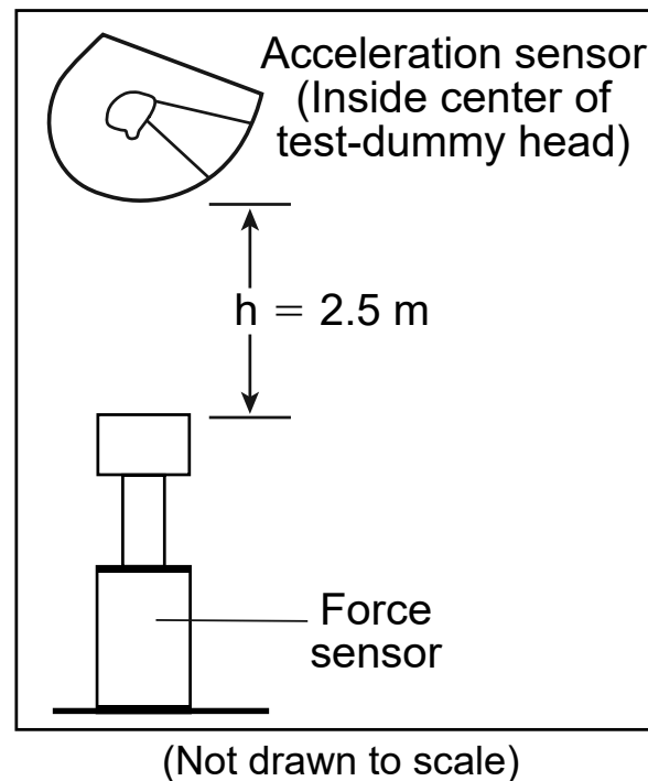
Diagram 2: Helmet Evaluation Test Setup
