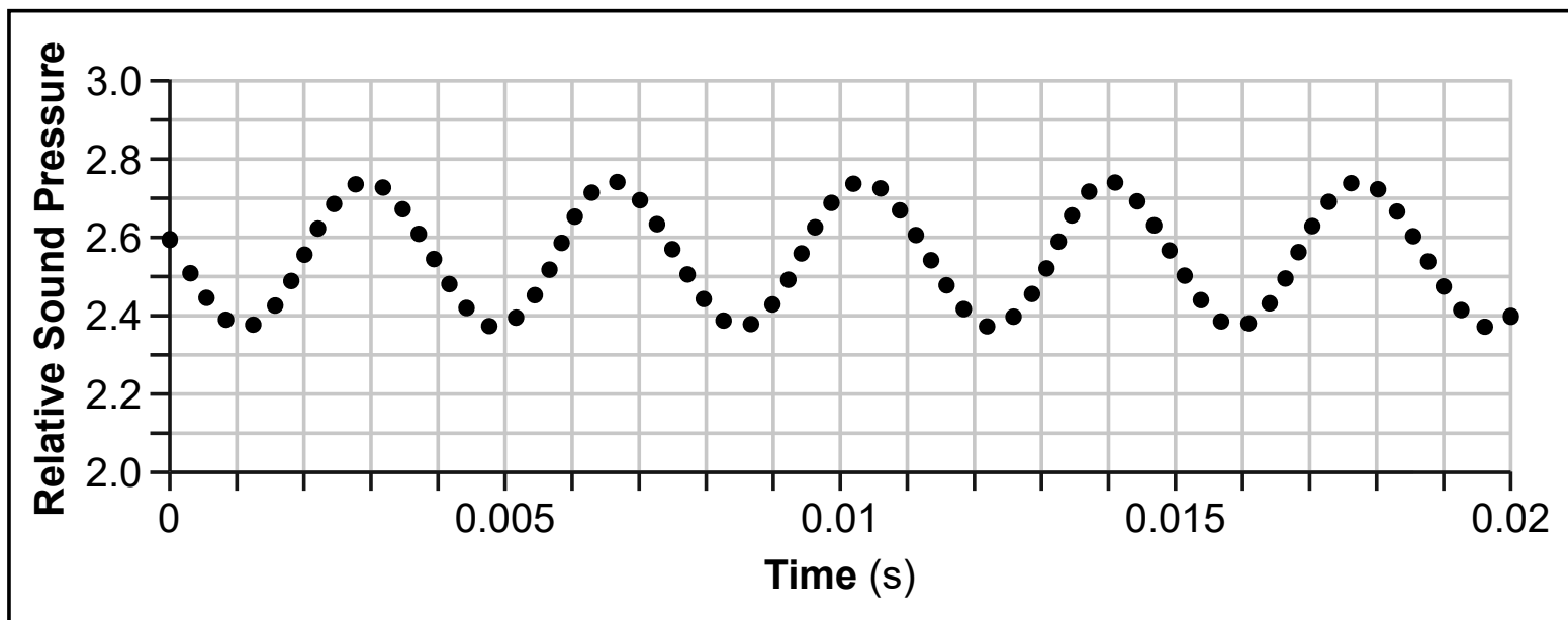
Graph 2: Tuning Fork Data for 0.0002-second Sampling Time
