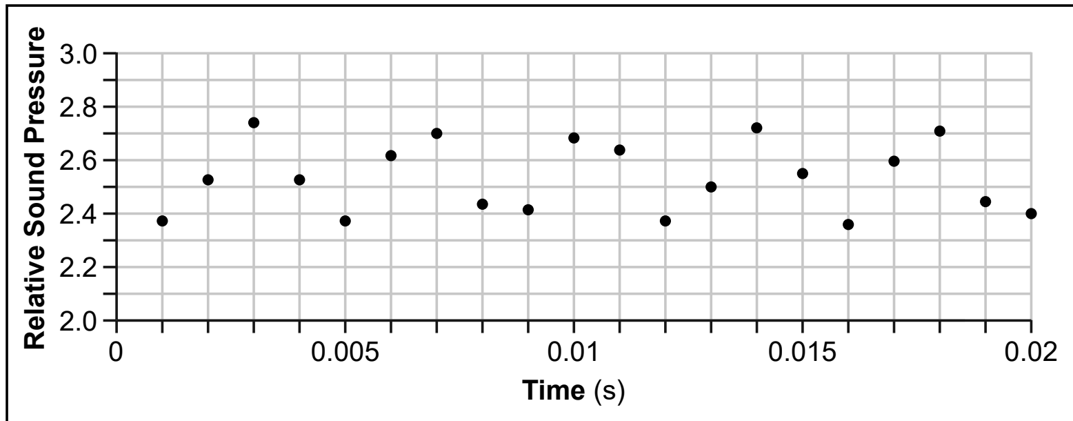
Graph 1: Tuning Fork Data for 0.001-second Sampling Time
